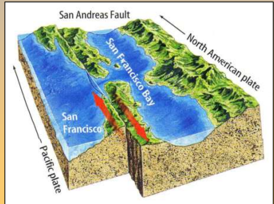
Movement between the 2 plates at the San Andreas Transform Fault. McGraw Hill/Glencoe, 1 st ed., pg. 146 (with permission). Table of Contents 20
