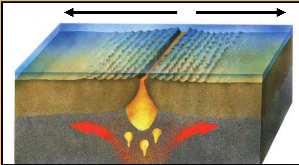
Sea-floor spreading at an oceanic divergent boundary.
